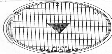
68-71 Inside Triangle was vertical base with 3/8" or 1/2" at bottom 5 3/4" Dia
